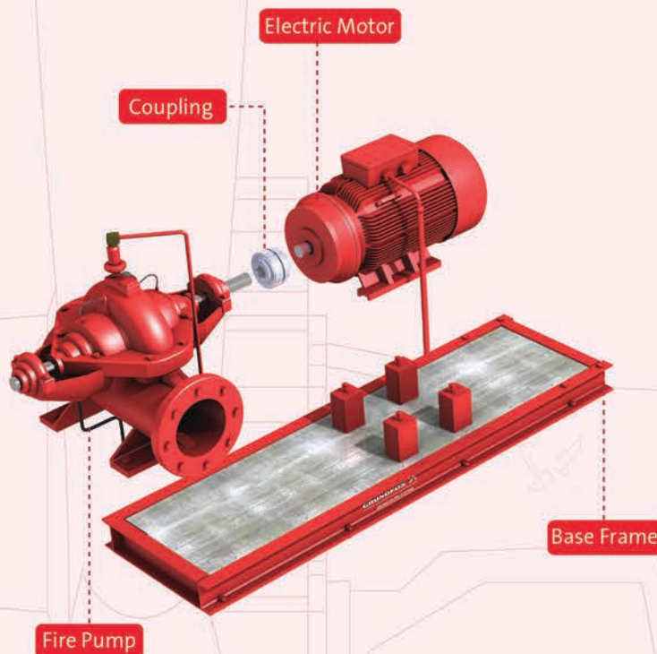
ELECTRIC FIRE PUMP (Exploded view)
