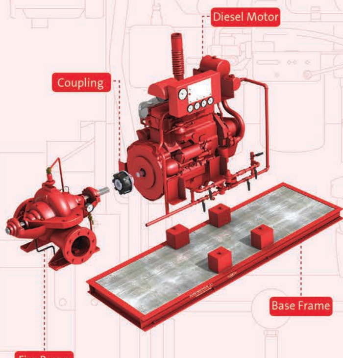
DIESEL ENGINE (Exploded view)
